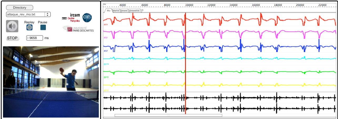
Fig. 0 : Screenshot of the interface developed for visualizing the measures and aligned media tracks. The top six curves are accelerations and angular velocities for X, Y and Z axis respectively. The waveform of the audio recording is visible at the bottom. The red cursor allows to scroll forward and backward while all tracks are played synchronously. Control panel is visible at top left and video window at bottom left.
